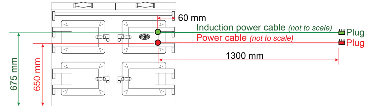
EVH 110i cable lengths
