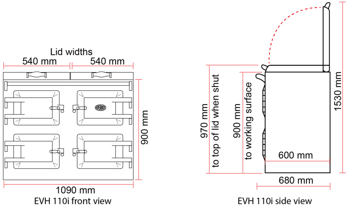
EVH110i dimensions
