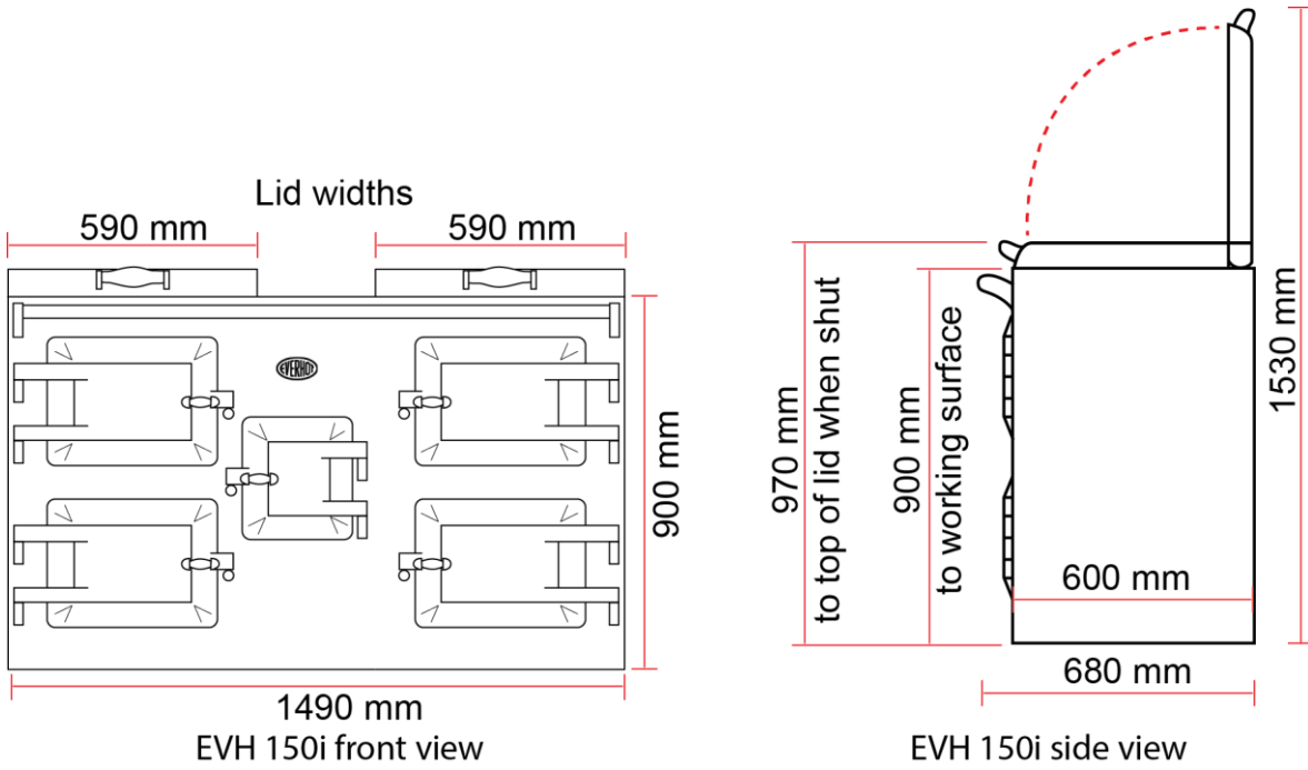
EVH150i dimensions
